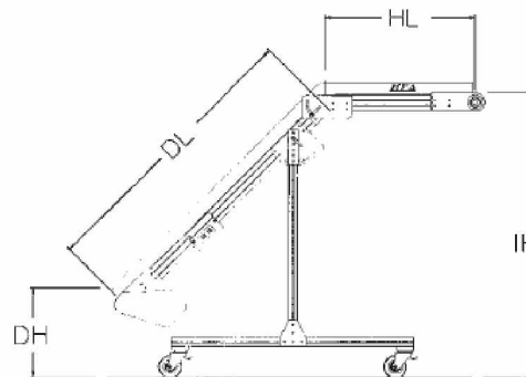
0-50° Angle Adjustment
